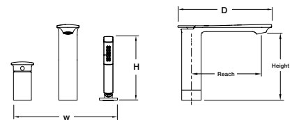
Deck-Mount Bath Faucet with Diverter/Handshower (W, D, H mm)
