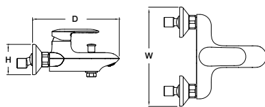
Exposed Bath and/or Shower Faucet (W,D,H mm)
